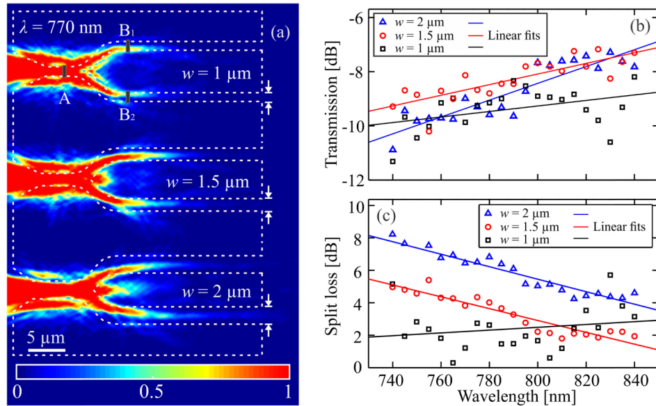
Fig. 8. (a) LRM image of the intensity distribution of three waveguides of different widths with Y-splitters at an excitation wavelength of 770 nm. (b) Transmission and (c) Y-splitter losses of the three structures in the wavelength range of 740–840 nm.
